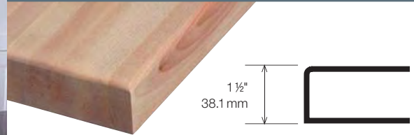
Profil 90° ( rayon = 1/4" ) / 90° Round Over (radius = 1/4")
